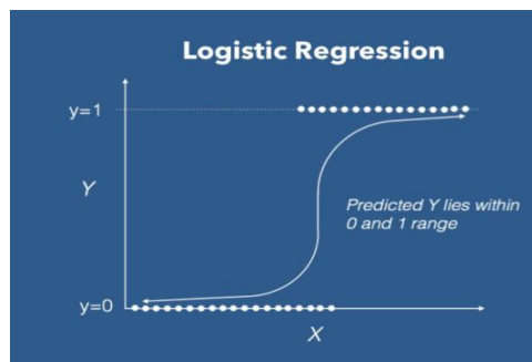
Fig.2 Logistic regression
