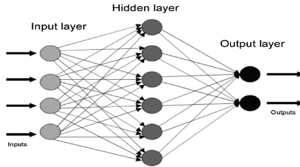
Fig.1 Neural Network
